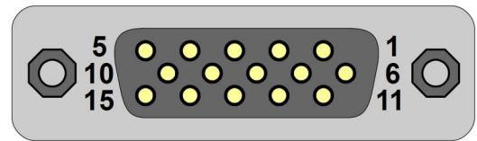
Figure 1: Option Modules connector
