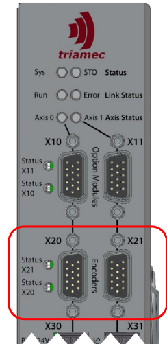
Figure 16: Encoder jack (X20,X21)
