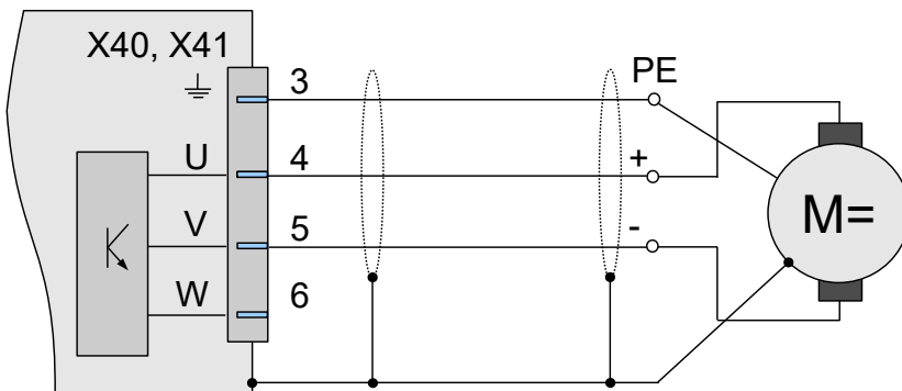
Figure 29: DC-motor connection
