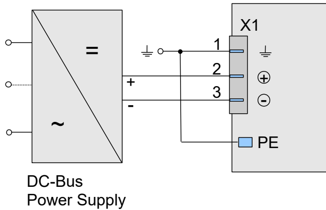
Figure 5: DC-Bus connection
