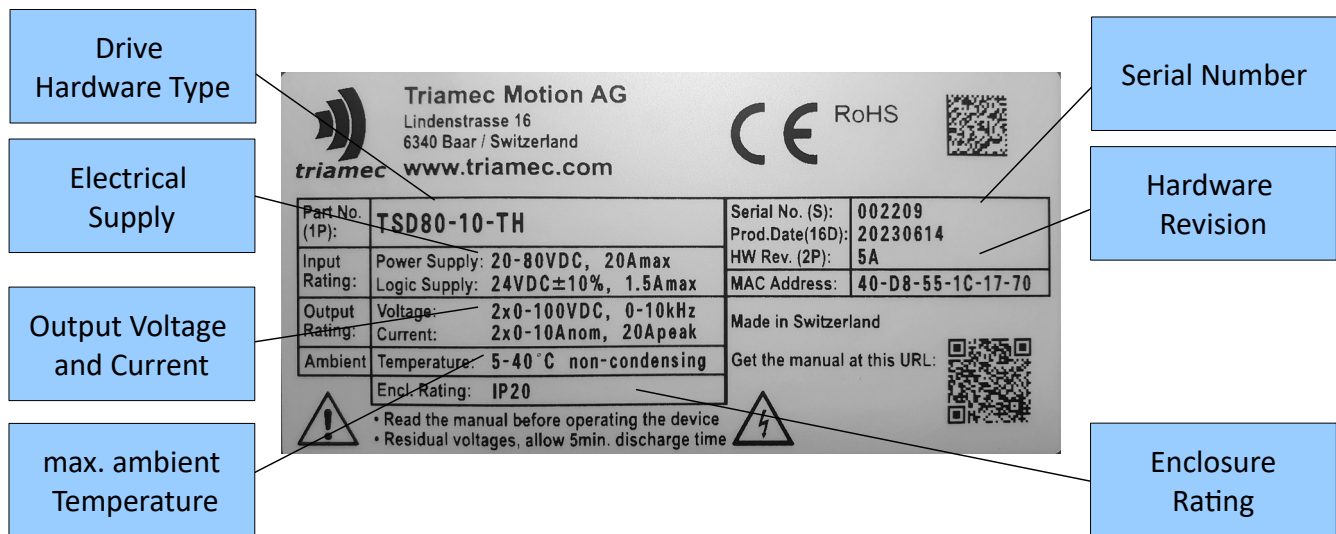
Figure 1: Nameplate of the TSD series servo drives
