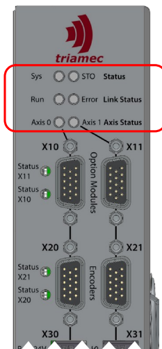
Figure 32: Status indicators
