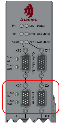
Figure 19: Encoder jack (X20,X21)
