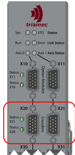
Figure 20: Encoder jack (X20,X21)
