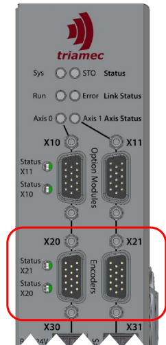
Figure 17: Encoder jack (X20,X21)
