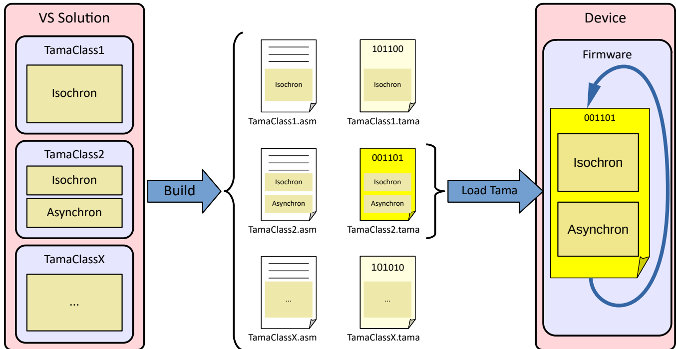
Figure 6: Build and load Tama Programs.
