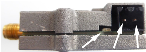
Power LED +24V GND
