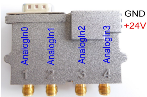
Figure 6: TAM register assignment with AN option module
