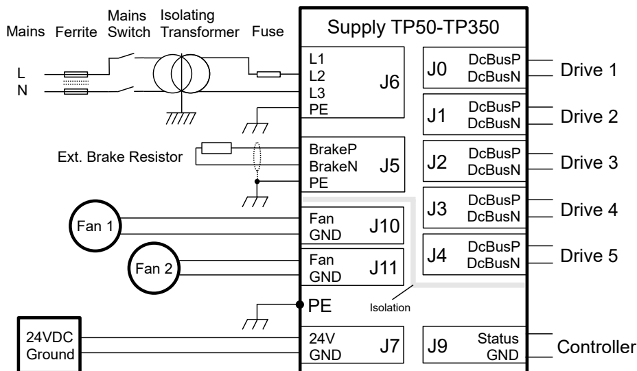
Figure 3: TP connections in case of 1 phase AC supply configuration
