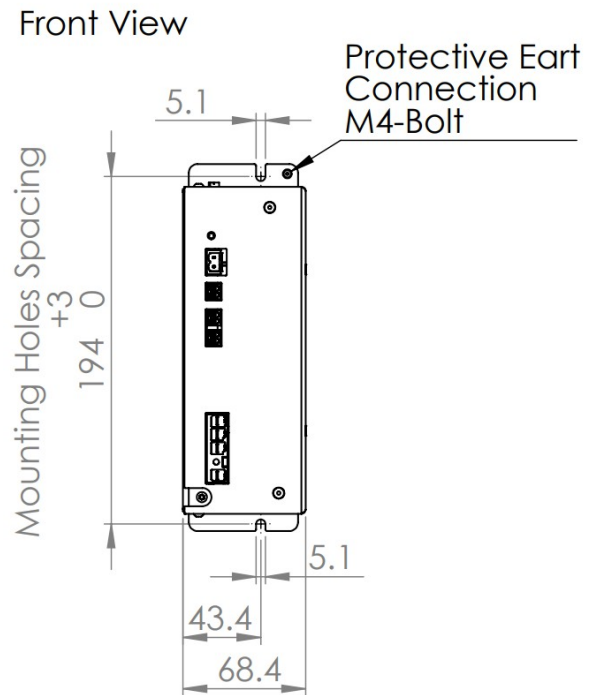
Figure 2: TP mounting dimensions
