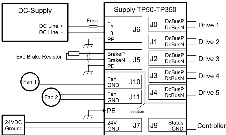
Figure 5: TP connections in case of DC supply configuration
