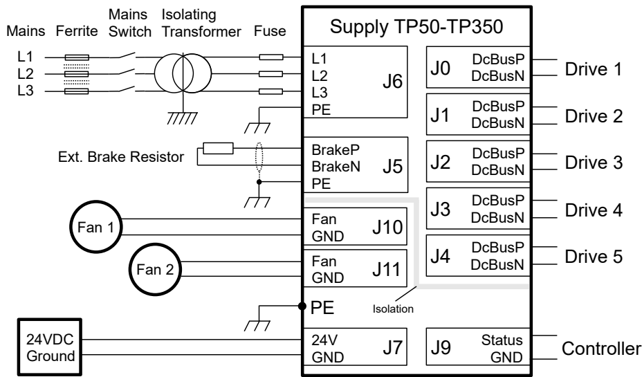
Figure 4: TP connections in case of 3 phase AC supply configuration
