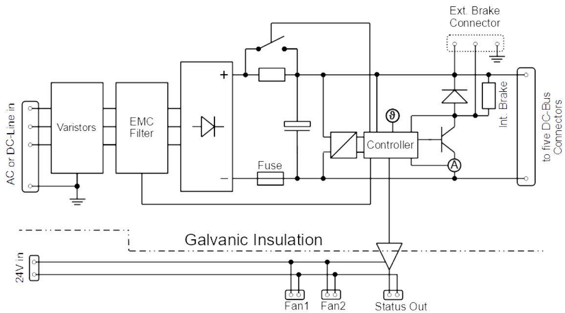
Figure 1: Block Diagram, Remark: As of hardware revision E5, there is no longer a fuse installed
