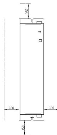
Figure 3: SP mounting Dimensions (Unit: mm)
