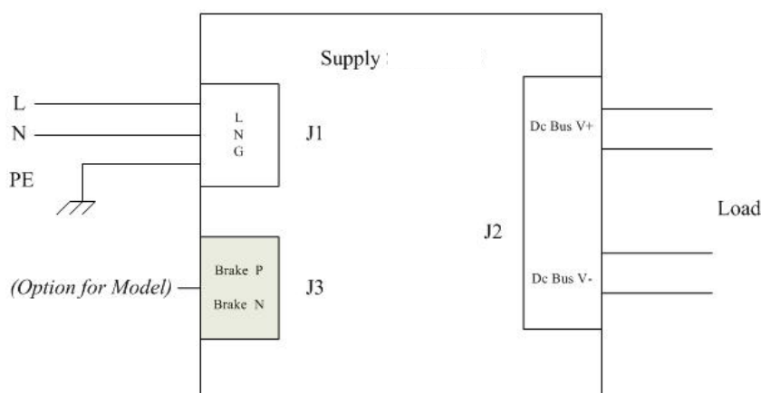
Figure 4: SP connections
