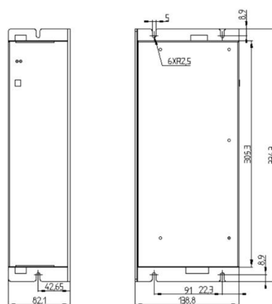
Figure 2: SP mounting Dimensions (Unit: mm) (Front View)
