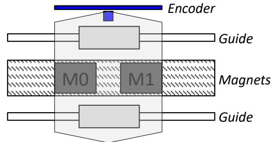
Figure 2: Linear Example Setup
