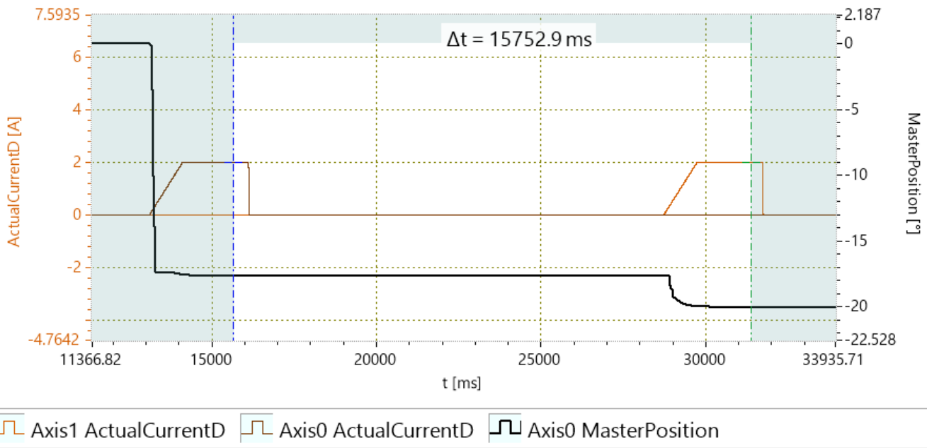
Figure 5: Phasing Offset Measurement
