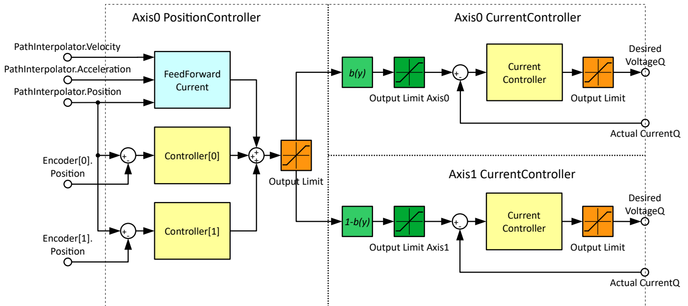
Figure 3: Block Diagram of the Controller Structure
